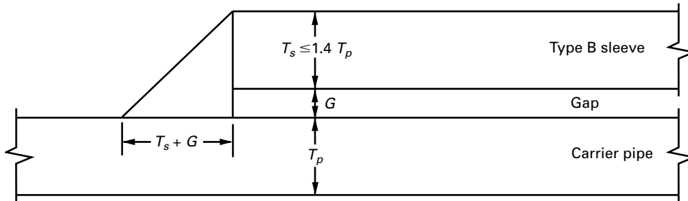
(18) Figure 206-3.5-1 Type B Sleeve Fillet Weld Size for Sleeve Thickness Less Than or Equal to 1.4 Times the Carrier Pipe Thickness
