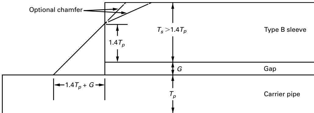
(18) Figure 206-3.5-2 Type B Sleeve Fillet Weld Size for Sleeve Thickness Greater Than 1.4 Times the Carrier Pipe Thickness
