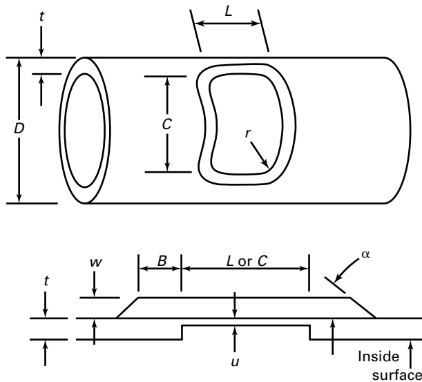
Figure 202-3-1 Weld Buildup Profile
